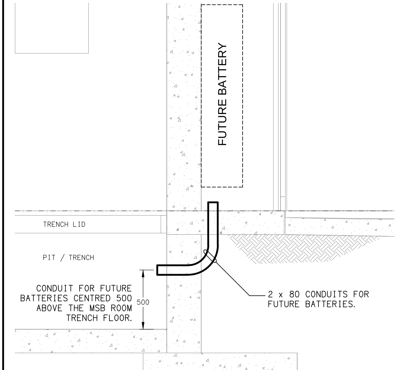
DETAIL A FUTURE BATTERY CONDUIT SECTION SCALE 1: 20
